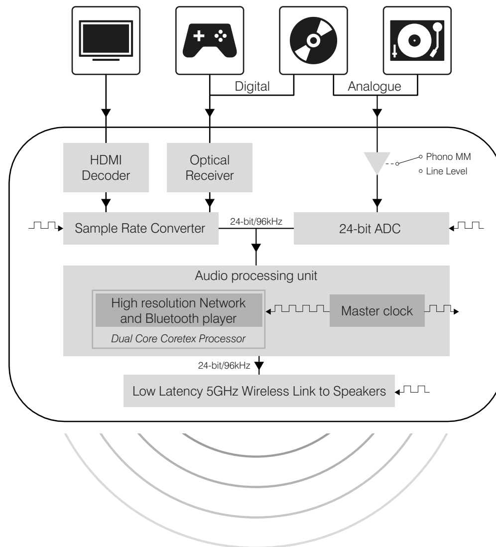
Figure 15: Hub detail diagram
