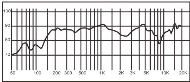
Frequency Response (dB SPL, 1W, 1m)
