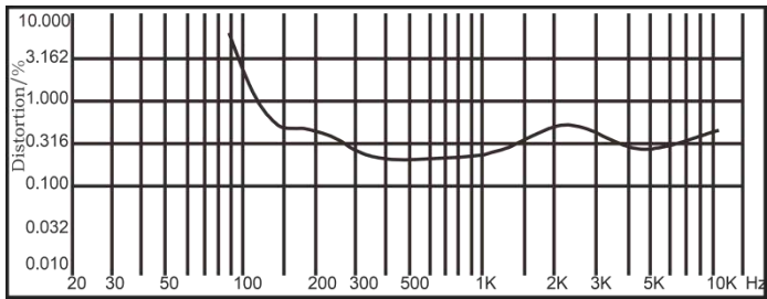
Distortion (THD<1.5% 1W, 1m, 200Hz-10kHz)
