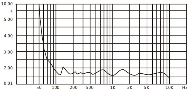
Distortion (THD<1.5% 1W, 1m, 100Hz-10kHz)
