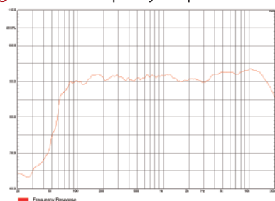
⊙ Artist T65 Frequency Response Curve
