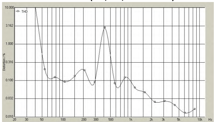
THD < 1.5% (1W, 1m, 60Hz-10kHz)
