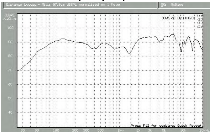
Frequency Response
