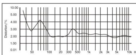
DSP455II Distortion
