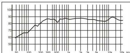
DSP255II Freq.Response (dB SPL, 1W, 1m)
