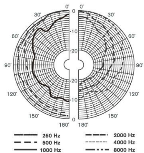
DSP8062 Horizontal directivity pattern
