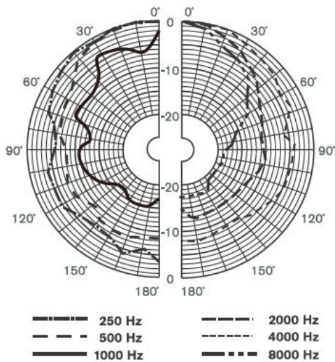
DSP8062 Vertical directivity pattern
